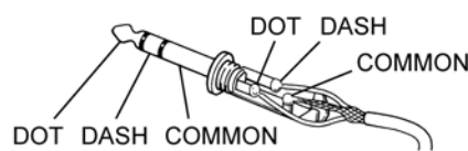
When connecting an electronic keyer paddle
